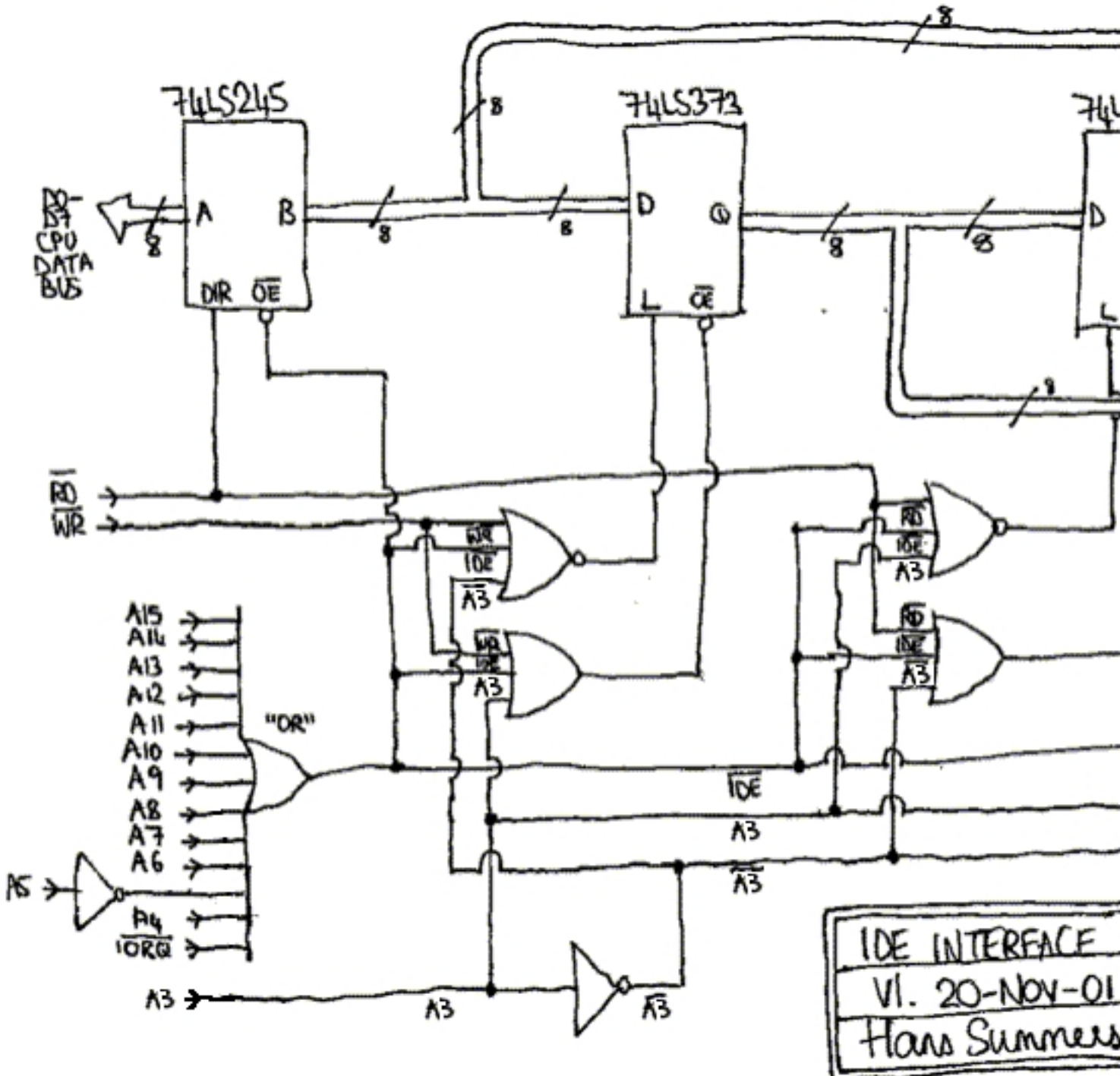
Figure 15: IDE interface and CPU Data Bus and CPU Address Bus connections to IDE registers. Written by Hans Summers
